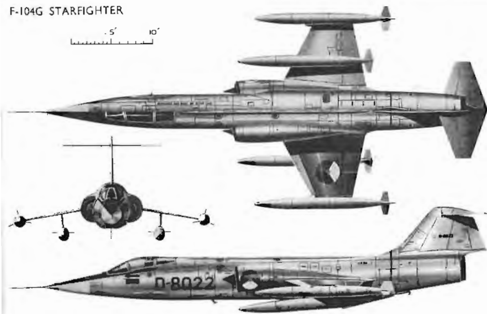
F-104G STARFIGHTER
